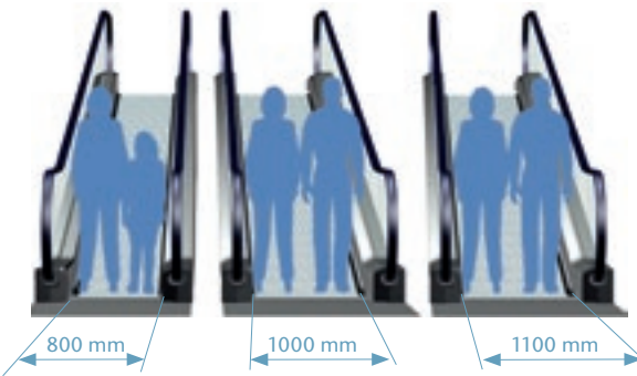
Figure 5.6 Inclined autowalk pallet widths
