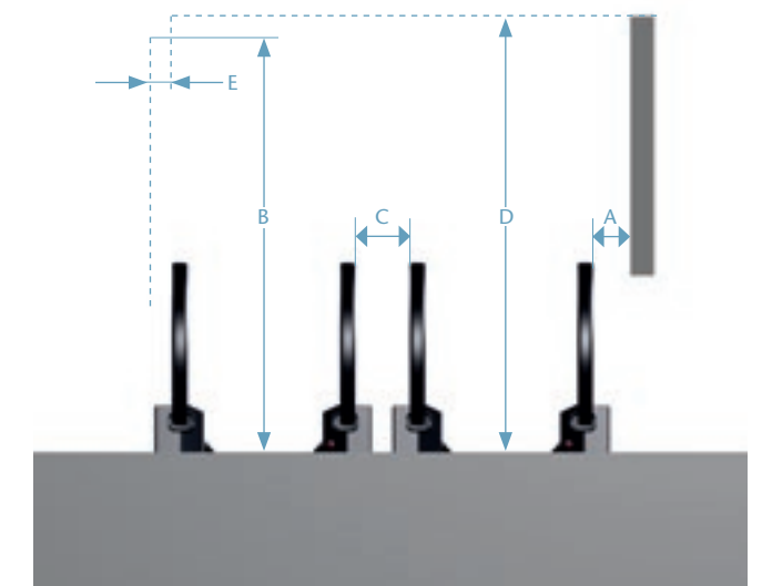
Figure 6.3 Minimum free area around escalators and autowalks
