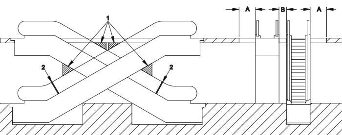
Figure 6.12 Head guards for criss-cross escalators
