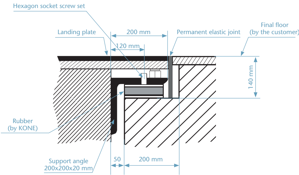
Figure 7.1 Escalator mounting angle
