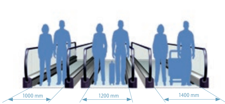
Figure 5.5 Horizontal autowalk pallet widths
